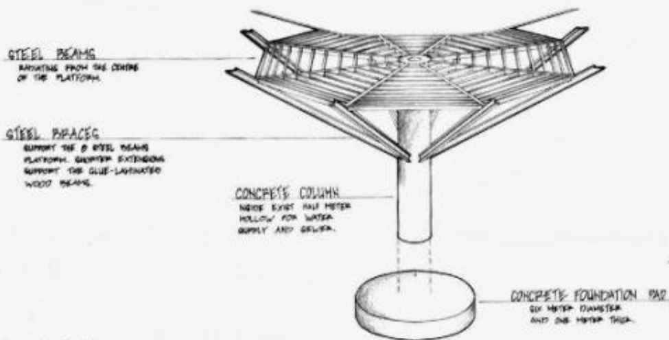
JOHN LAUTNER CHEMOSPHERE AXONOMETRIC (S T R U C T U R E)
